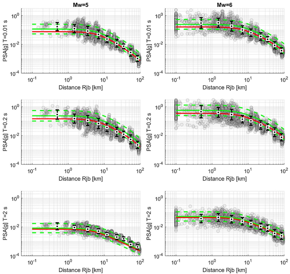
Fig. 9 Simulated spectral acceleration (PSA) for M_w=5 (left) and M=6 (right) as a function of the Joyner-Boore distance ( R_{jb} ) for three spectral periods ( T=0.01 s, 0.2 s and 2 s). The gray circles represent the geometric mean of the horizontal components, and the vertical black bars represent the mean and standard deviation of simulated values over distance bins. Stations within the surface projection of the rupture are plotted at R_{jb}=0.1 km. The GMM for Italy (ITA18) by Lanzano et al. (2019a) is plotted in light green (median \pm 1 standard deviation) considering a V_{s30}=800 m/s and normal fault mechanism. The median ITA18ref (adjusted for reference rock conditions according to Lanzano et al. 2022) is shown in red
