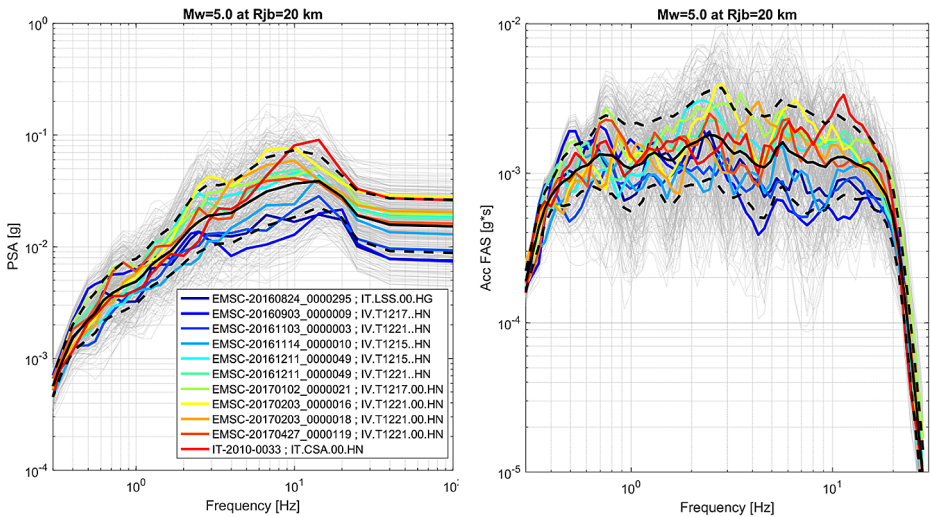
Fig. 12 (Left) simulated response spectra (in gray) for the M_w=5 scenarios at 20 km (stations at distances between 15 km to 25 km are used) for the geometric mean of horizontal components. The mean \pm 1 standard deviation of the simulated spectra is shown in black. The mean spectrum obtained for each EGF in shown in color. (Right) the same as in the left panel but in terms of Fourier amplitude spectra (FAS)
