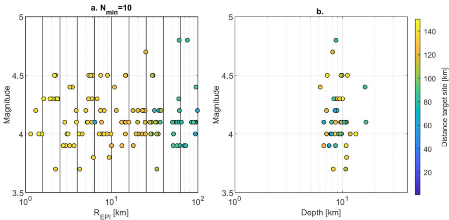
Fig. 3 (a) The magnitude-distance distribution of selected recordings to construct the database for EGF simulations ( \text{DATA}_{\text{EGF}} ). (b) Magnitude-depth distribution of these recordings. The color scale represents the distance to the target site. N_{\min} indicates that distance bins have been filled, whenever possible, by recordings from different stations until a minimal number of 10 recordings is reached
