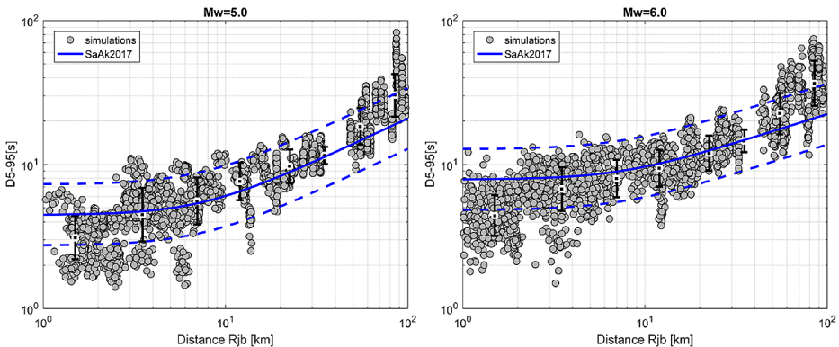
Fig. 13 Comparison between simulated horizontal significant durations (D5-95: time elapsed between 5% and 95% of the total Arias Intensity) as a function of distance for M_w=5 (left) and M_w=6 (right) scenarios and the predictions by the Sandikkaya and Akkar (2017) empirical model for the Pan-European region (in blue, median \pm 1 standard deviation) for V_{s30}=800 m/s and normal-fault mechanism
