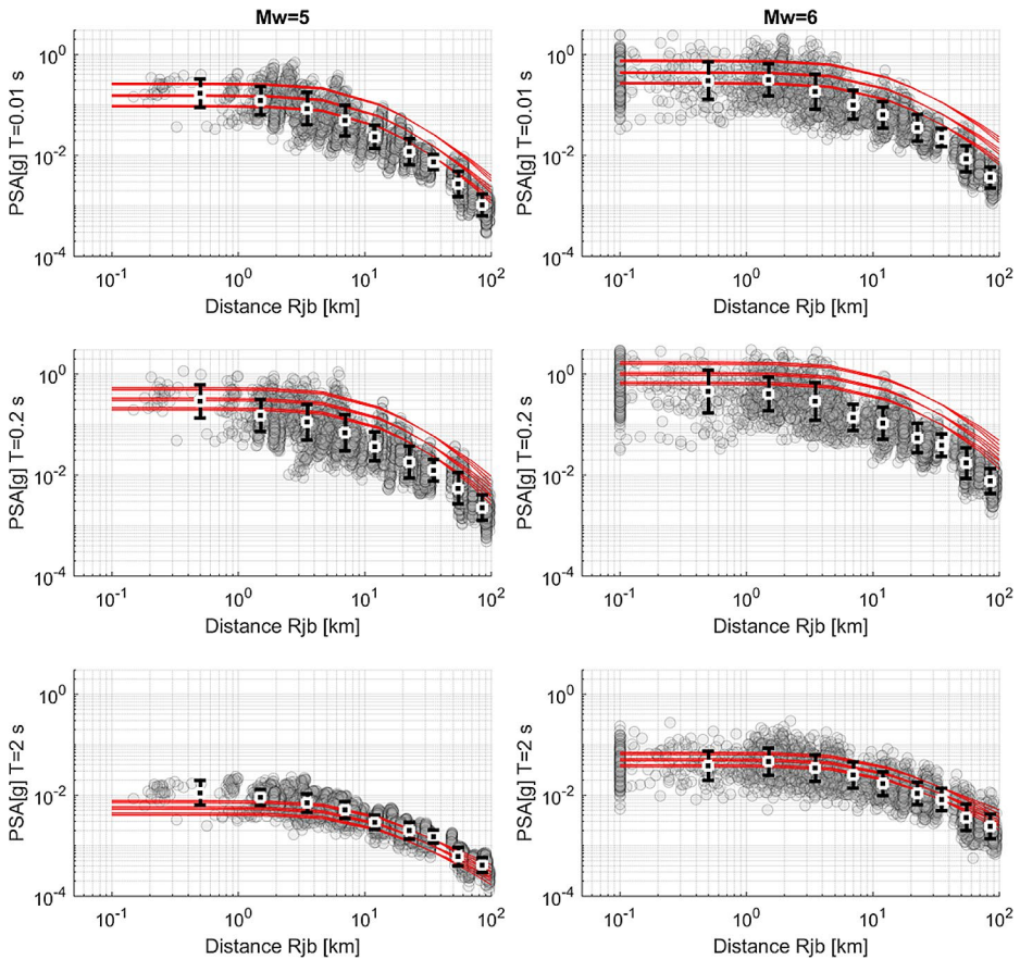
Fig. 10 Simulated spectral acceleration (PSA) for M_w=5 (left) and M_w=6 (right) as a function of the Joyner-Boore distance (Rjb) for three spectral periods ( T=0.01 s, 0.2 s and 2 s). The gray circles represent the geometric mean of the horizontal components, and the vertical black bars represent the mean and standard deviation of simulated values over distance bins. Stations within the surface projection of the rupture are plotted at R_{jb}=0.1 km. The European GMM adopted by Weatherill et al. (2020) is plotted in red for a V_{s30}=1100 m/s and considering the 9 branches of the logic tree proposed to capture uncertainties in median ground motion for attenuation cluster 3
